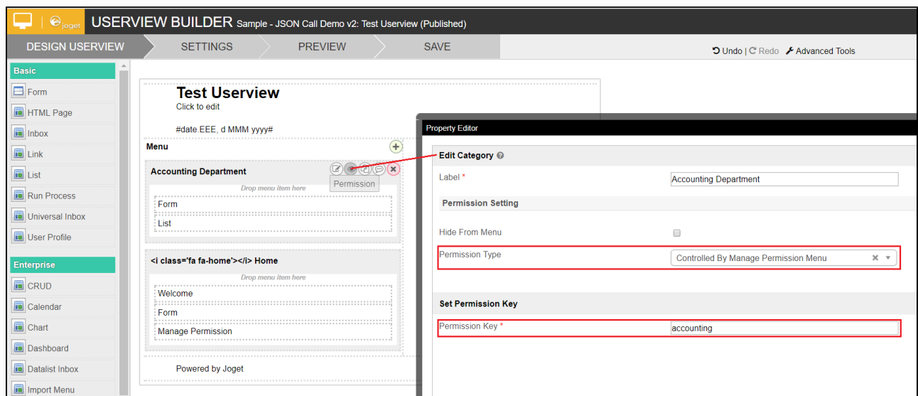
Figure 5: Adding permission to an userview category
