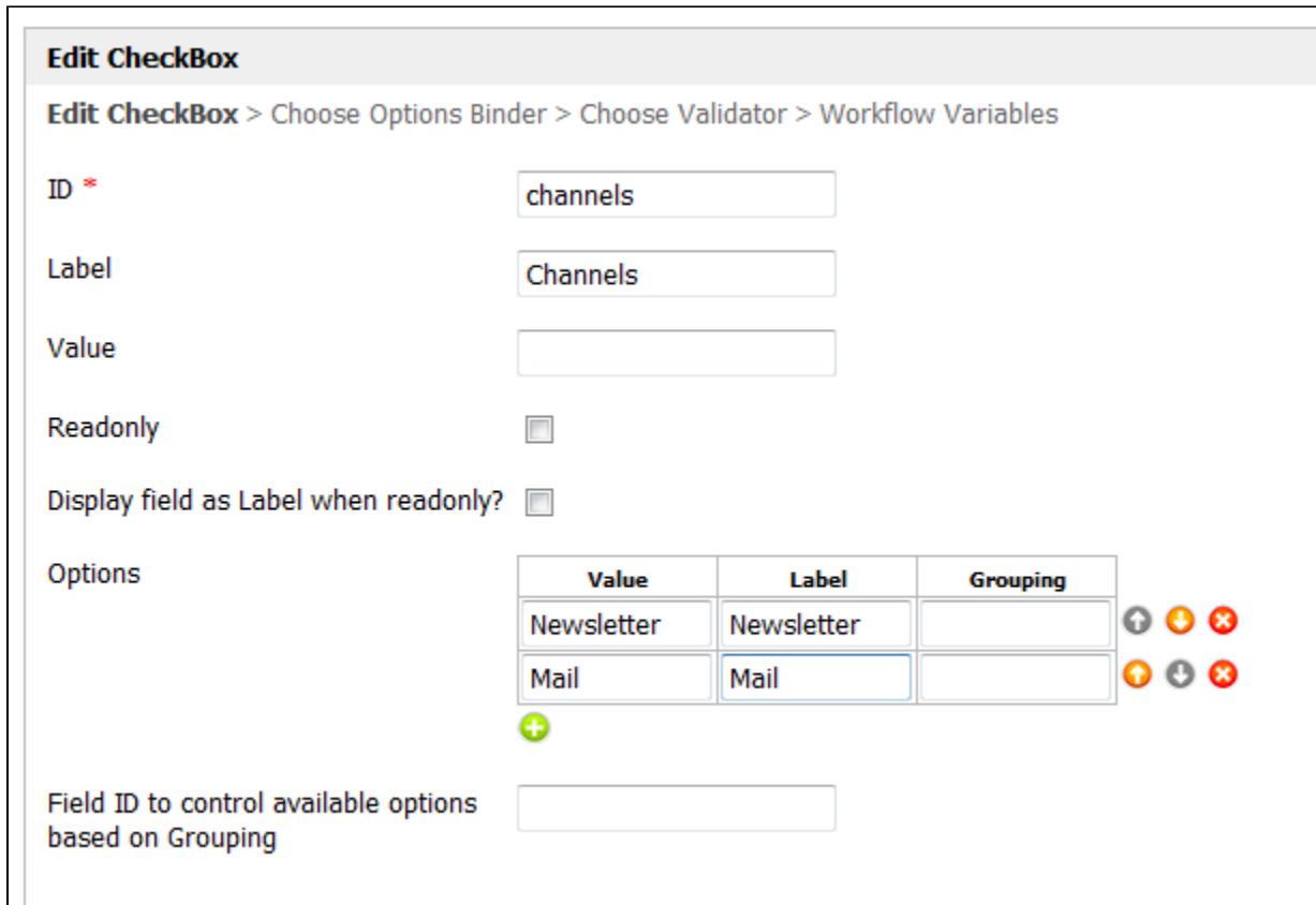
Figure 2: CheckBox Properties
