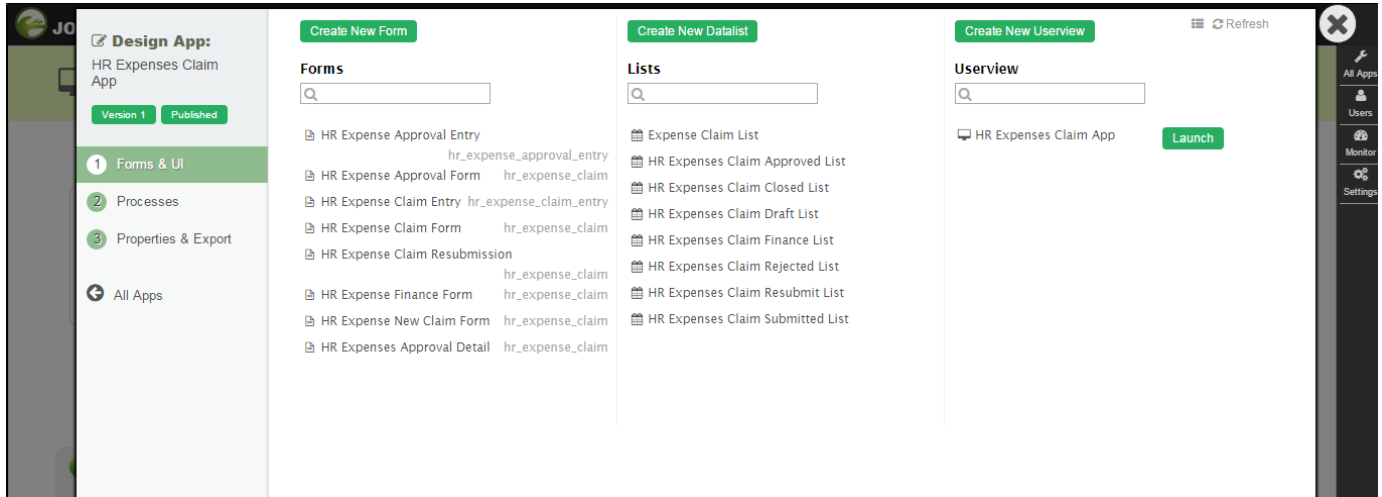
Figure 1: Forms & UI
