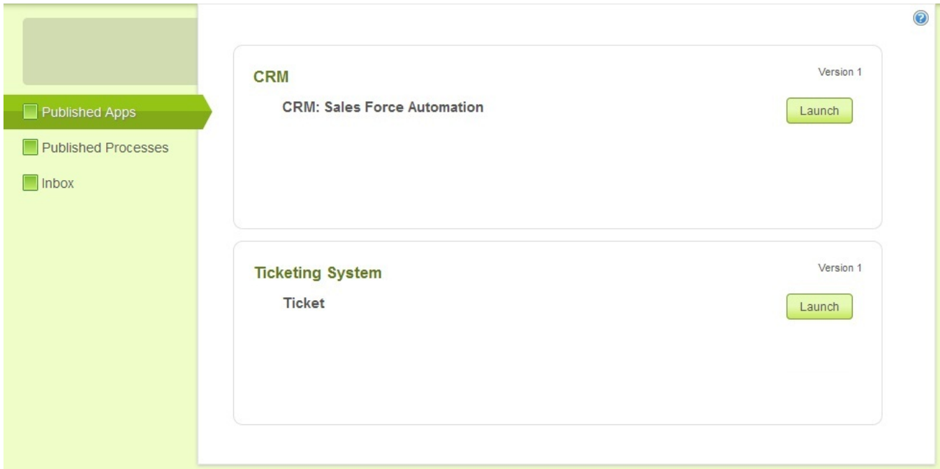
Figure 1: Published Apps
