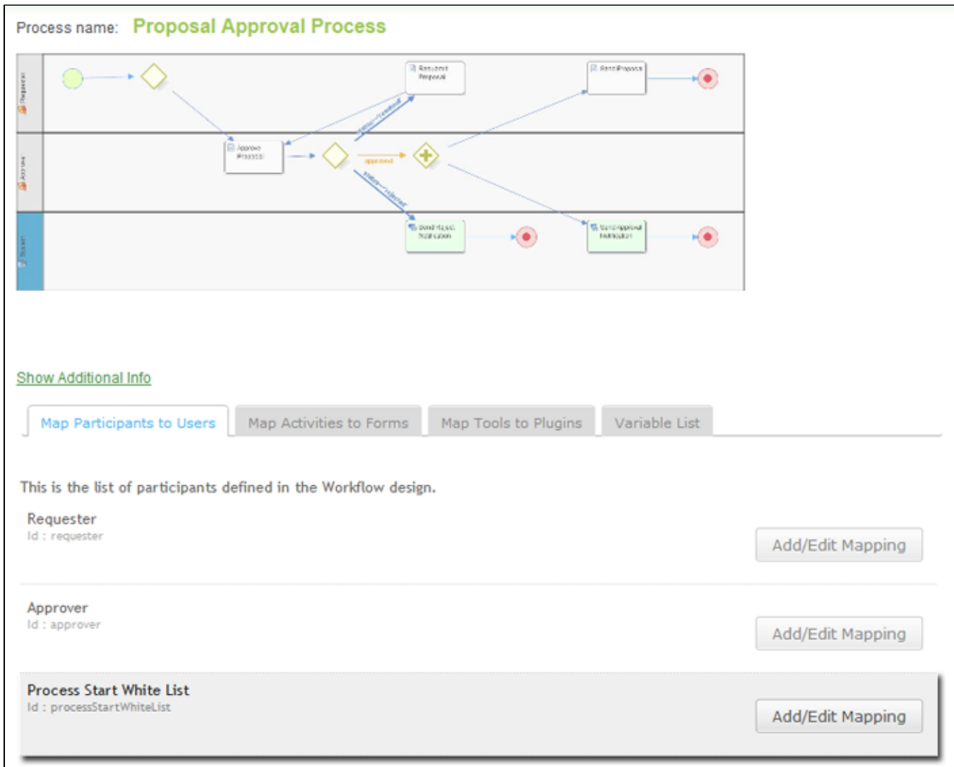
Figure 2: Process Start White List
