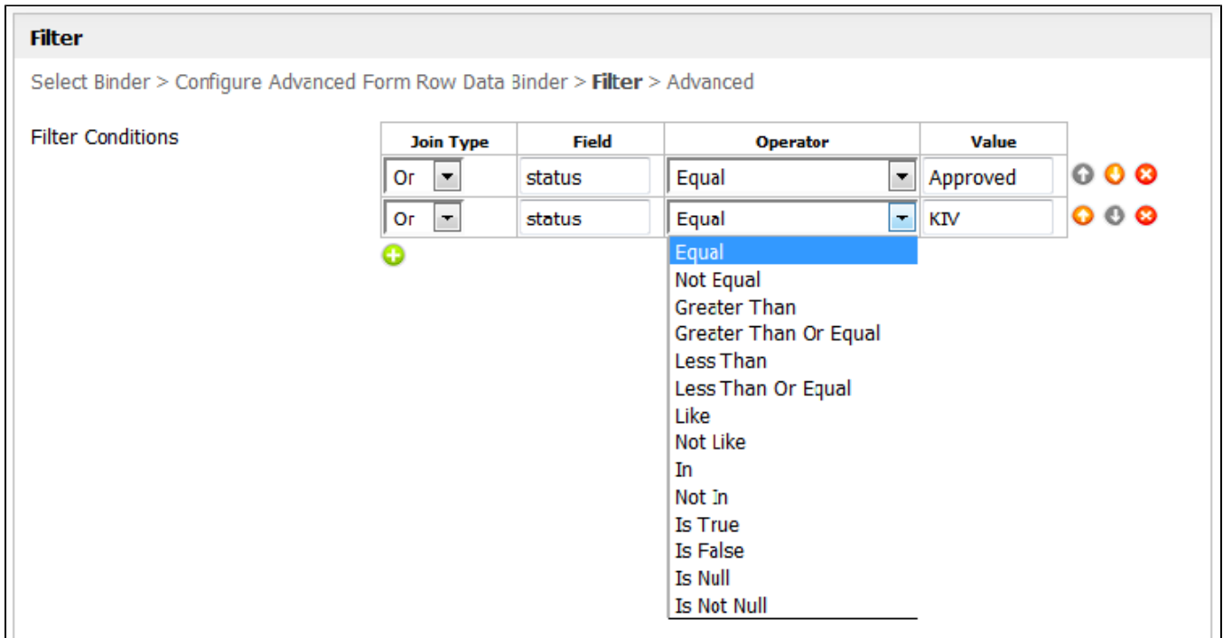
Figure 1: Filter properties in Advanced Form Row Data Binder
