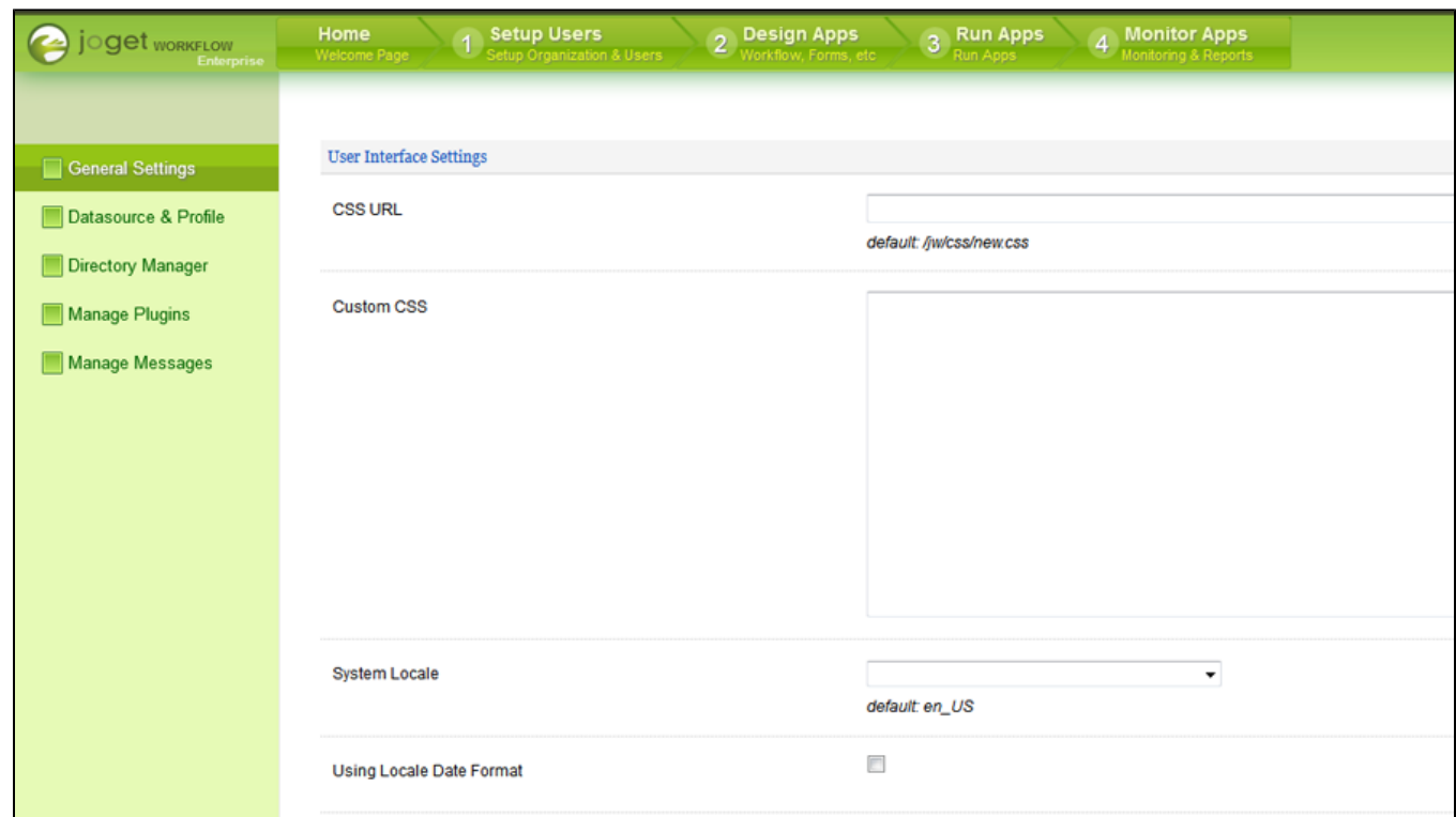
Figure 1: System Settings
