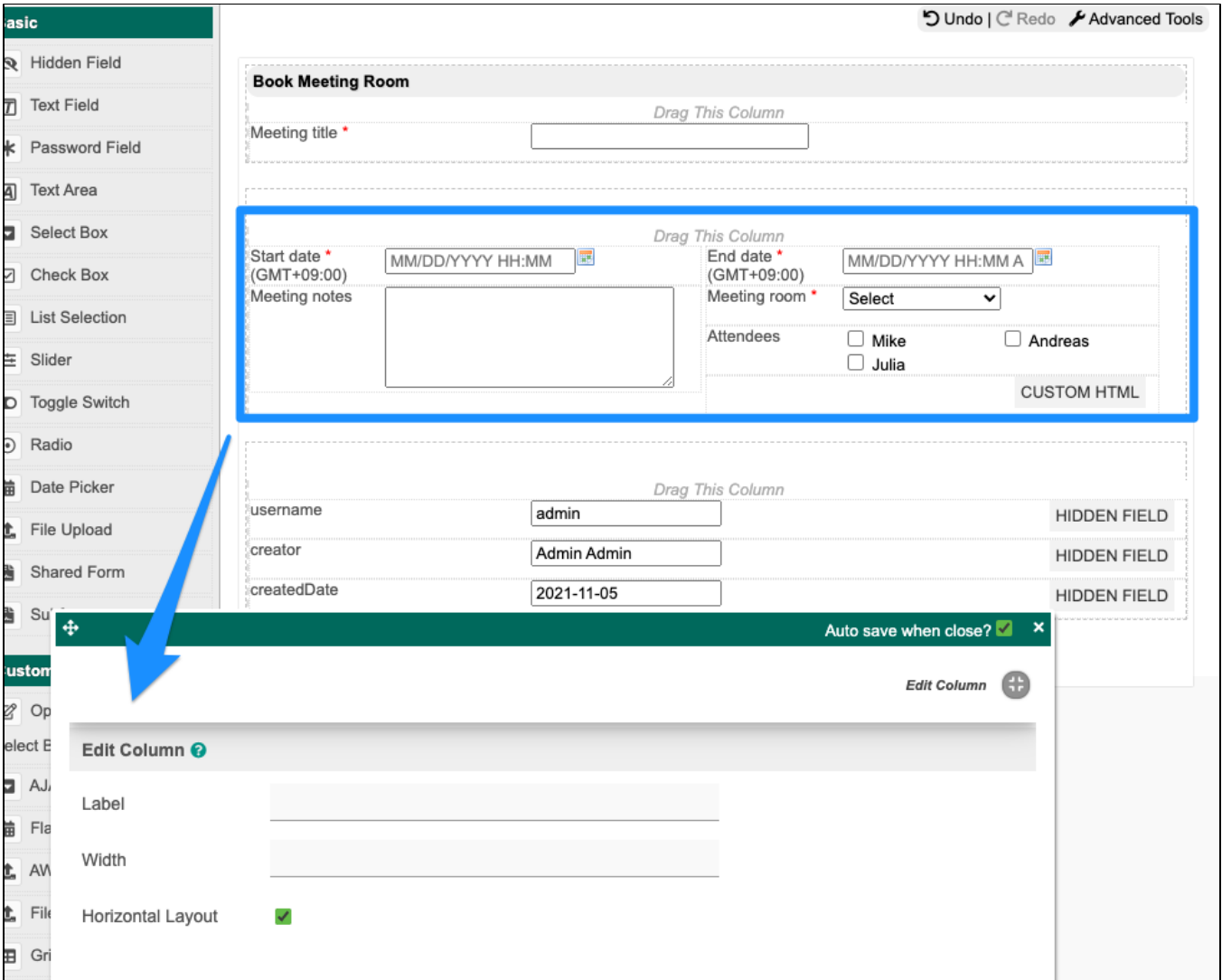
Figure 2: Column Properties as Horizontal Layout
