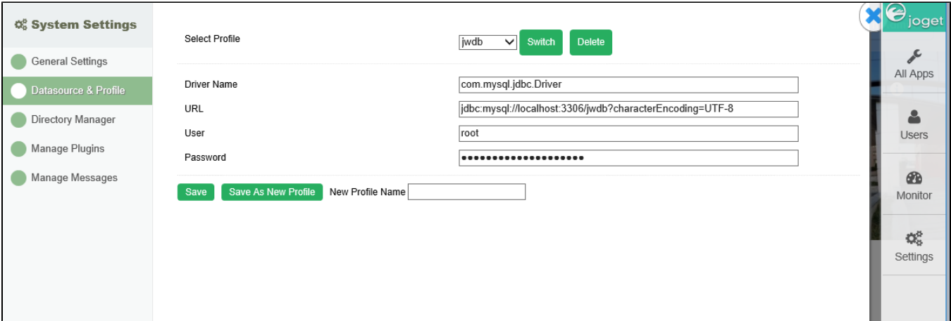
Figure 1: Datasource & Profile
