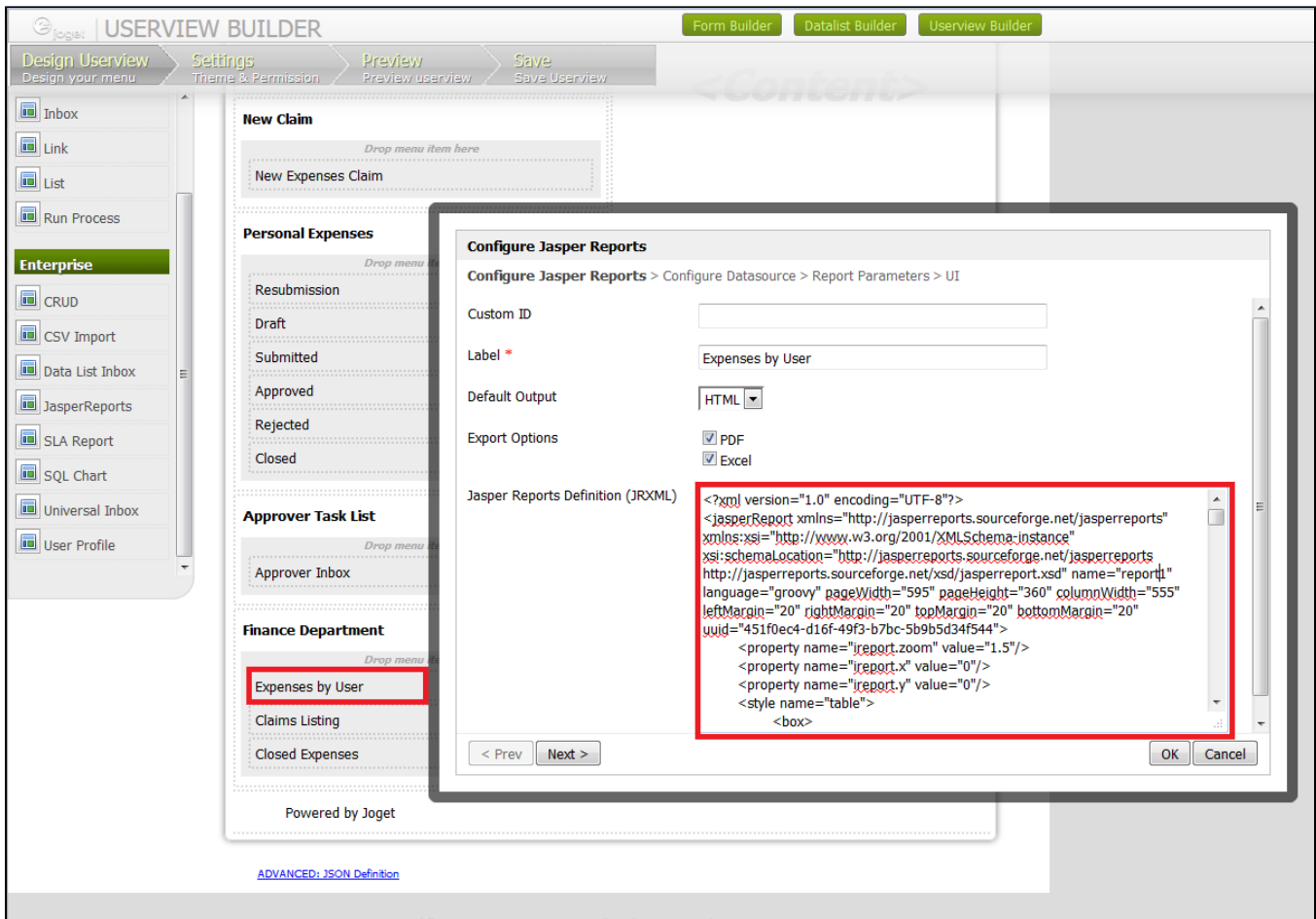
Figure 2: Adding the report definition into Joget Userview's Jasper Reports element
