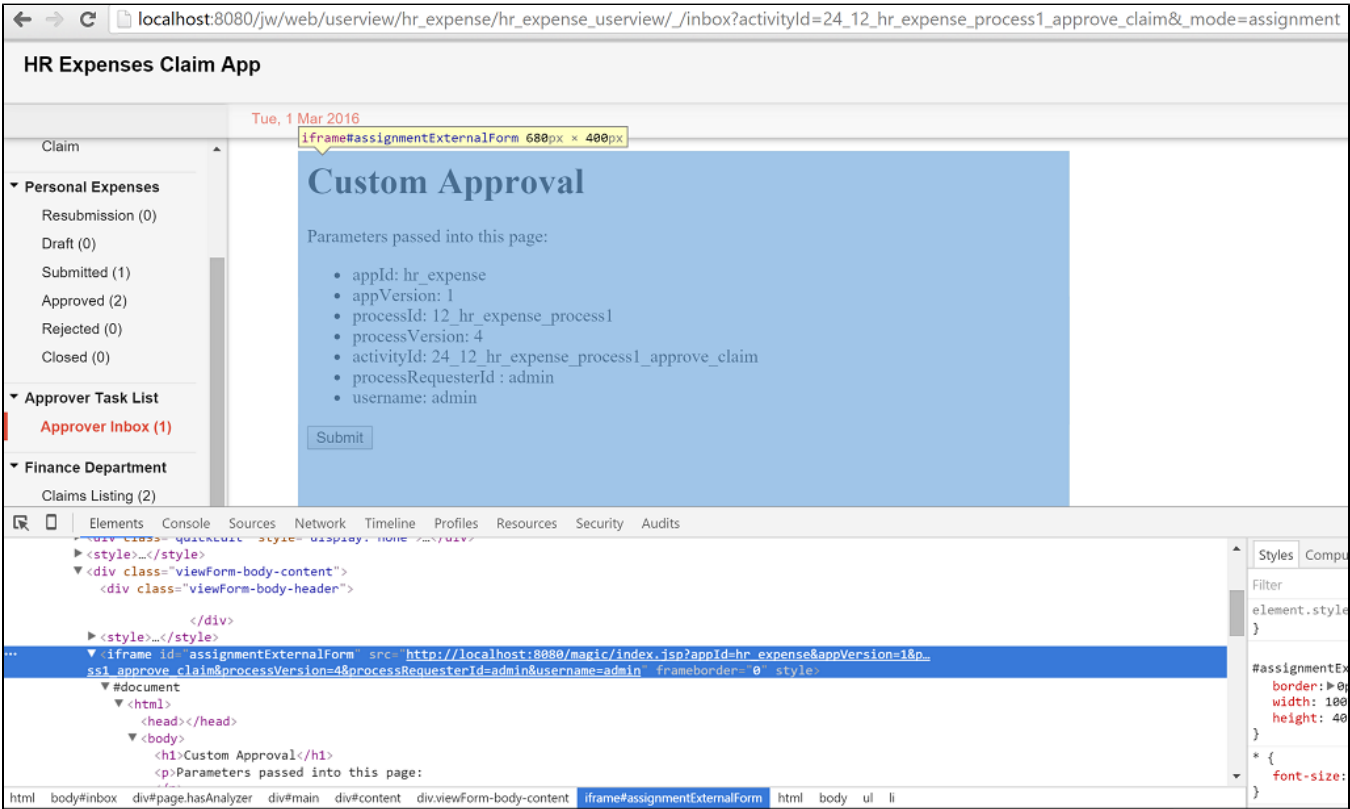
Figure 1: Inbox showing assignment that is mapped to External Form
